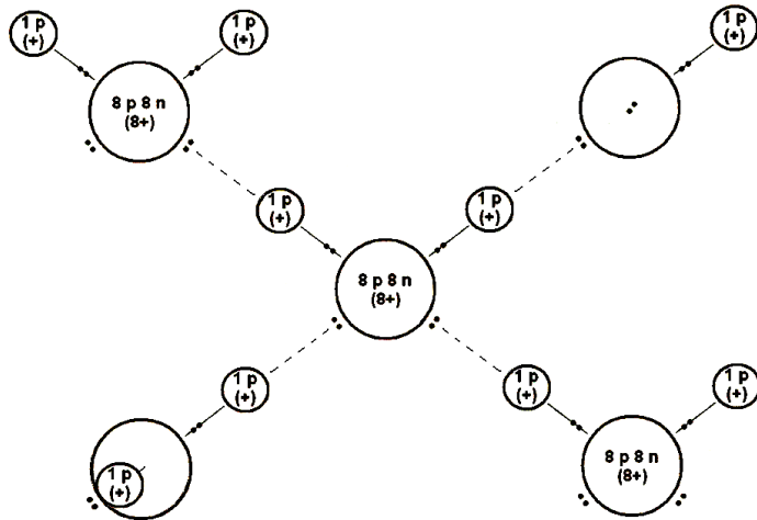
Figure 3. A schematic of water and its resulting formation of hydrogen bonds (dashed lines) The water molecules at the top right and bottom left are rotated on their bond axes away and toward the reader, respectively, to convey a sense of three-dimensionality.
