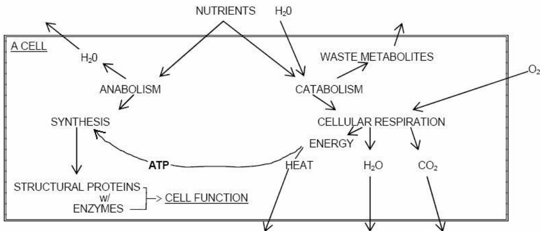
Figure 4. Summary of the Metabolic Processes in a Chemotroph
