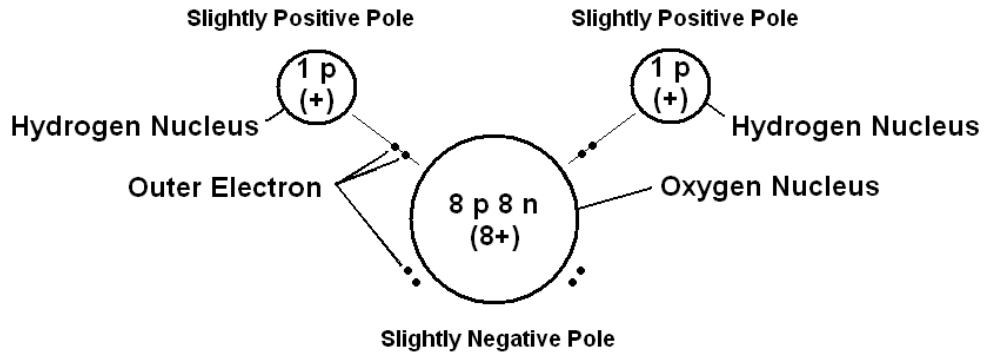
Figure 2. A schematic of the polarity of the water molecule.
